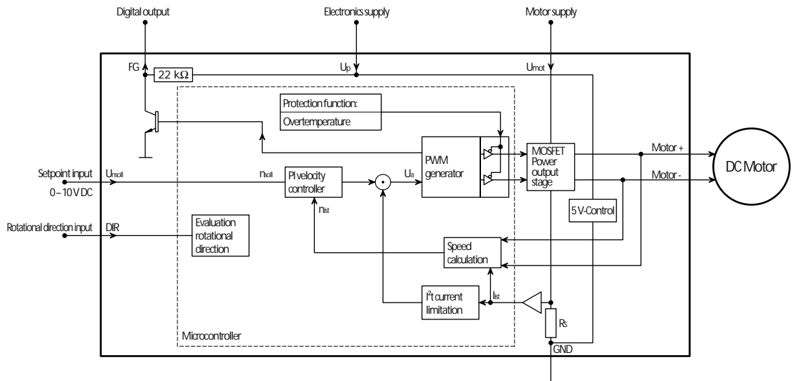
Block diagram:
