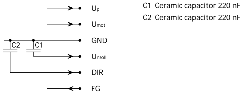
Circuit diagram 1
