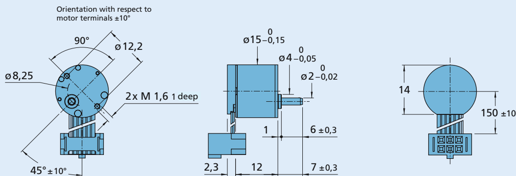
1512U...SR... IE2-8
