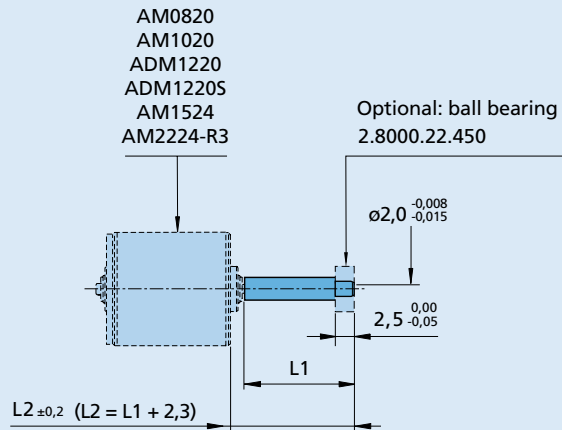
Version with bearing tip
